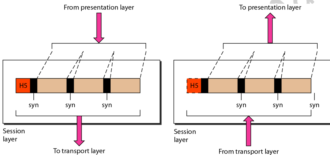
Figure 2.6 Session layer
