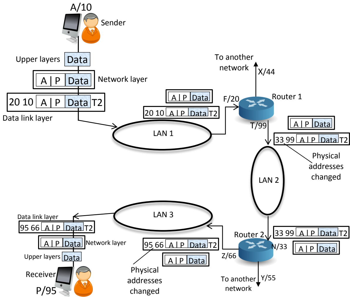
Figure 3.6 Example of logical (IP) addresses
