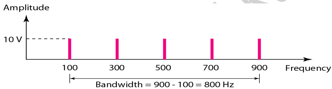
Figure 4.8 The bandwidth for Example 4
