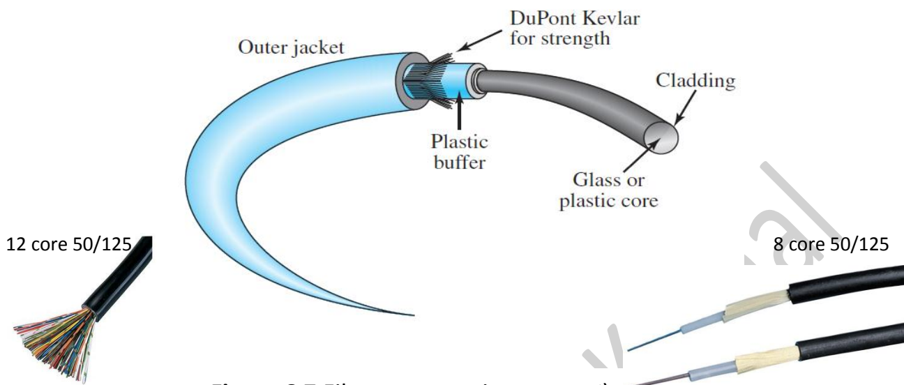
Figure 6.7 Fiber construction (للاطلاع فقط)
