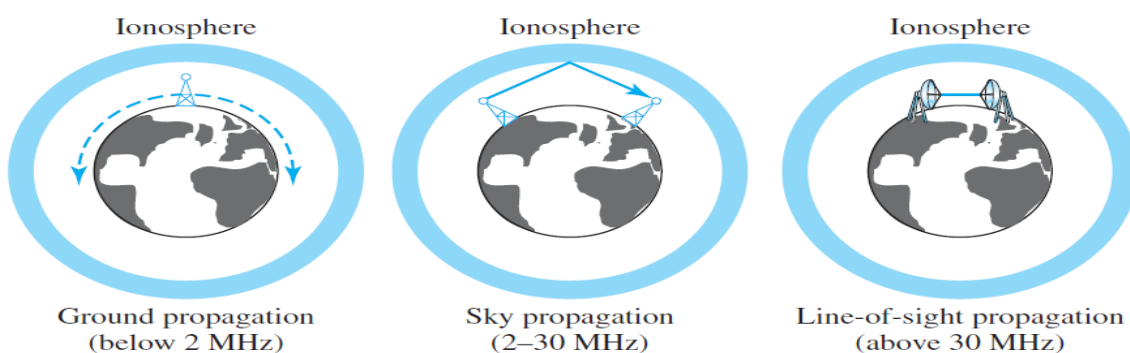
Figure 6.9 Propagation methods
