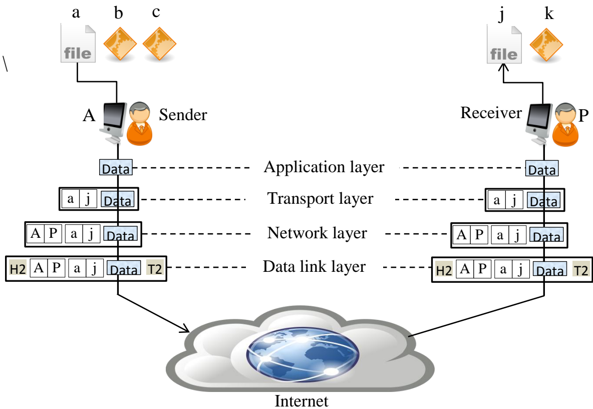
Figure 3.7 Example of port addresses
