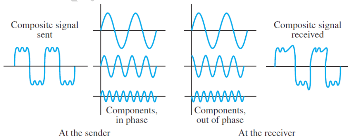
Figure 5.8 Distortion
