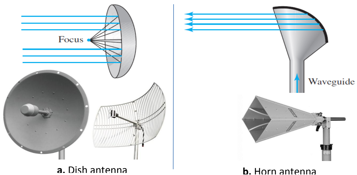
Figure 6.11 Unidirectional antennas
