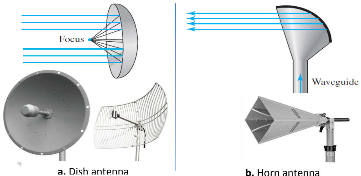
Figure 6.11 Unidirectional antennas
