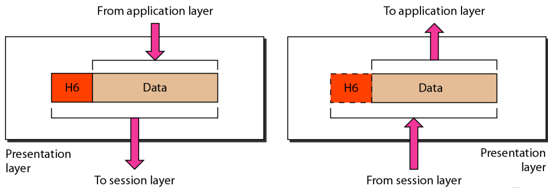
Figure 2.7 Presentation layer
