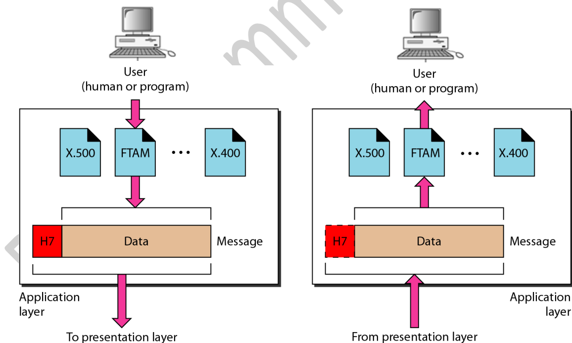
Figure 2.8 Application layer
