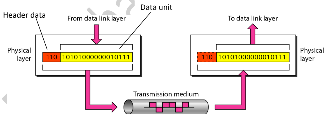
Figure 2.2 Physical layer
