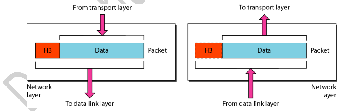
Figure 2.4 Network layer
