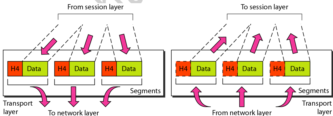
Figure 2.5 Transport layer
